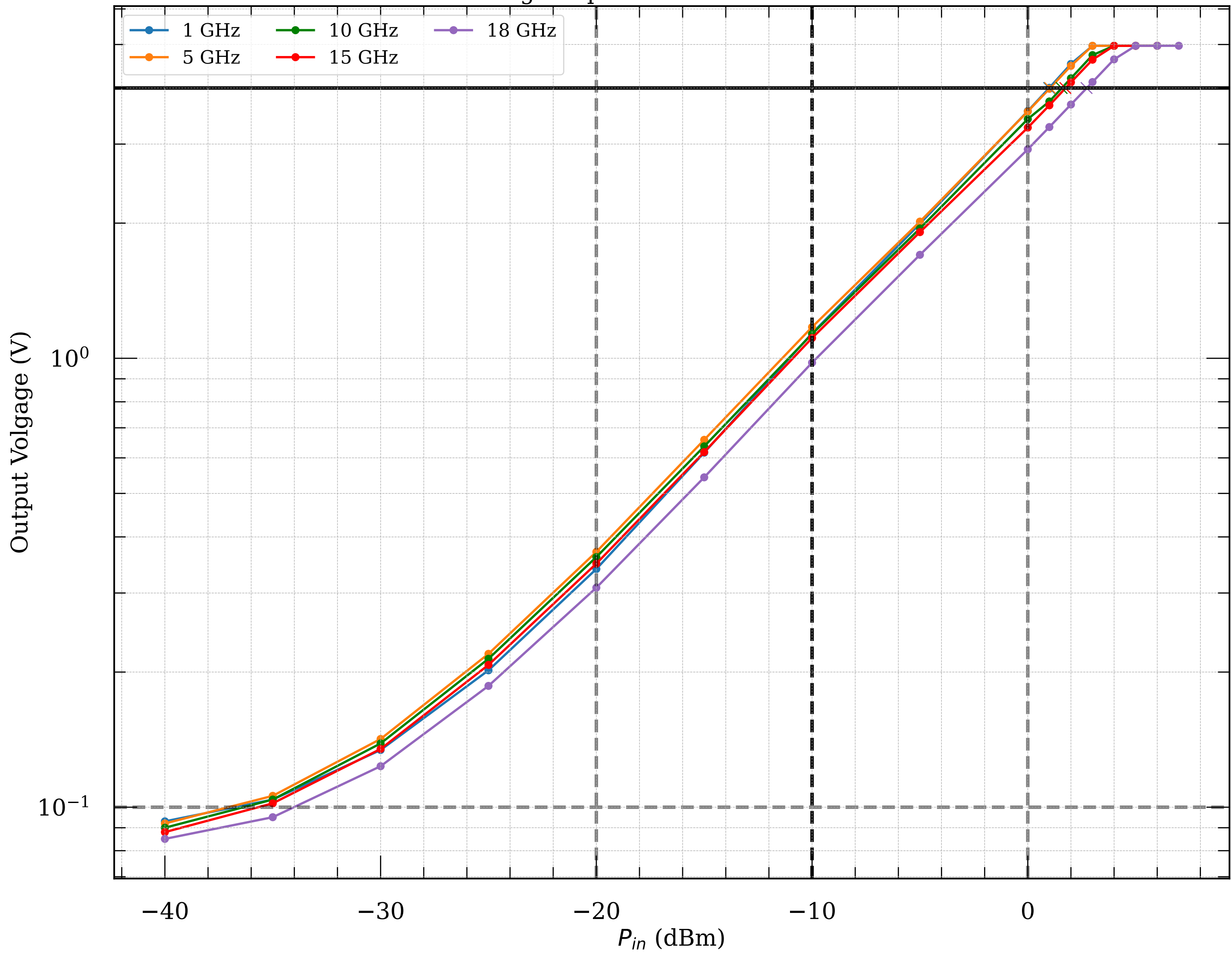
Measured voltage-to-power curve of detector module032
